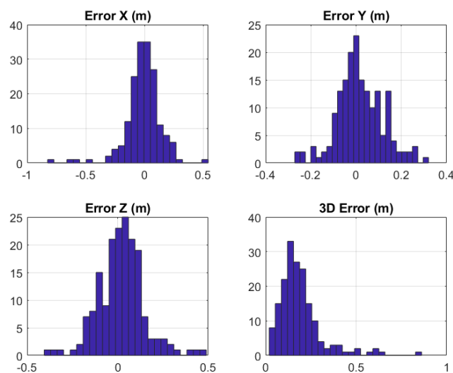
Figure 10: Simulation of Setup B with out Outliers
