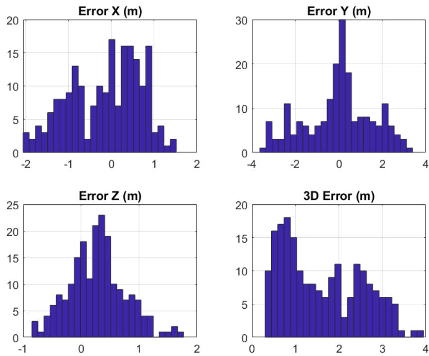
Figure 13: Positioning Error Profile of Simulation without Outliers in Setup A
