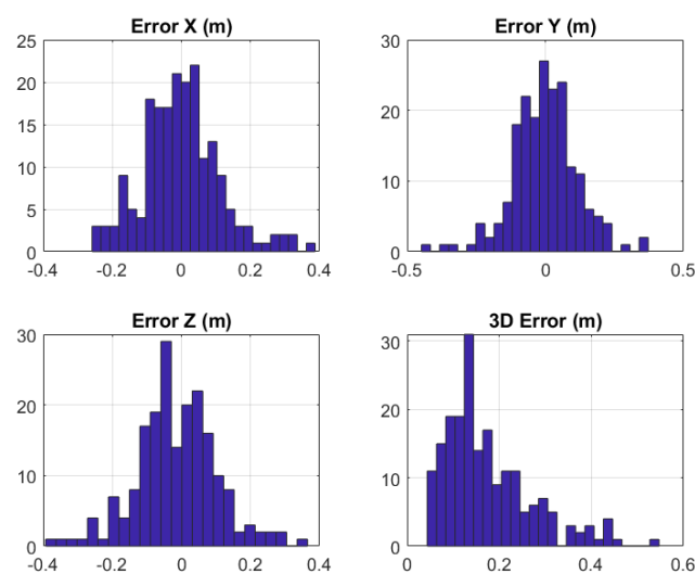
Figure 8: Simulation of Setup A with out Outliers
